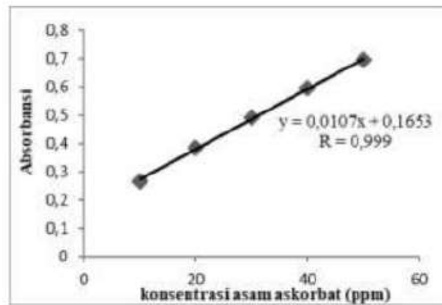
Figure 3. Ascorbic Acid Linear Regression Curve with Linear Regression Formula y = 0.0107 + 0.1653 and the value of r = 0.9999
